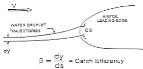
Figure 12: Graphic explaining how the collection efficiency ( \beta ) is calculated
