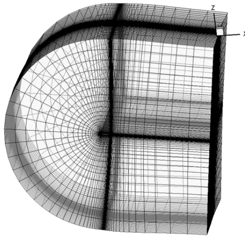
Figure 21: 131x90x45 C-H mesh produced using CGT
